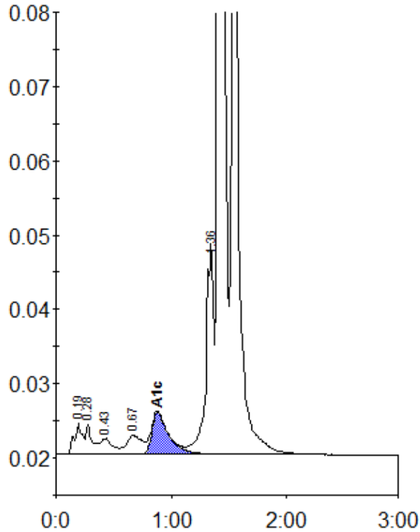
Peak table - ID: 10423653
